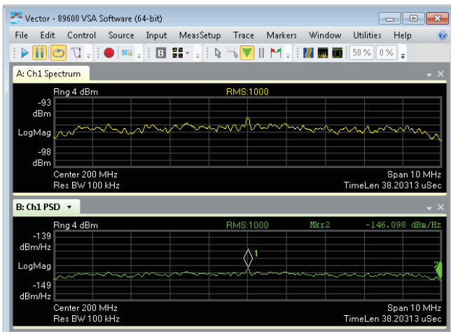
Figure 4. Noise power spectral density (NSD) measured with the 89600 VSA software on one channel of the M9703A. With a very low NSD down to -145 dBm/Hz, the M9703A has comparable performance to some 16-bit digitizers.
